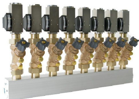
Photo - valve block VB2-020GA8 with valves and flow switch M101
