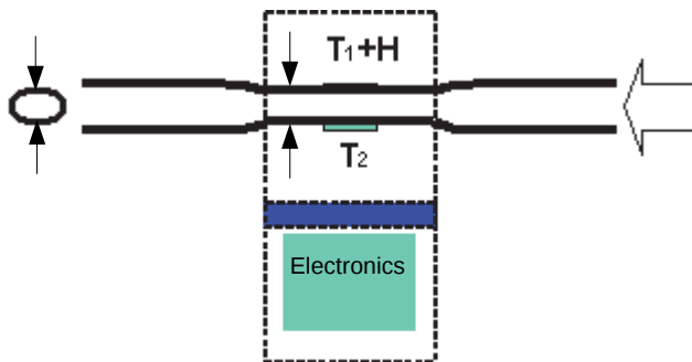
Plug-in sensor construction principle
